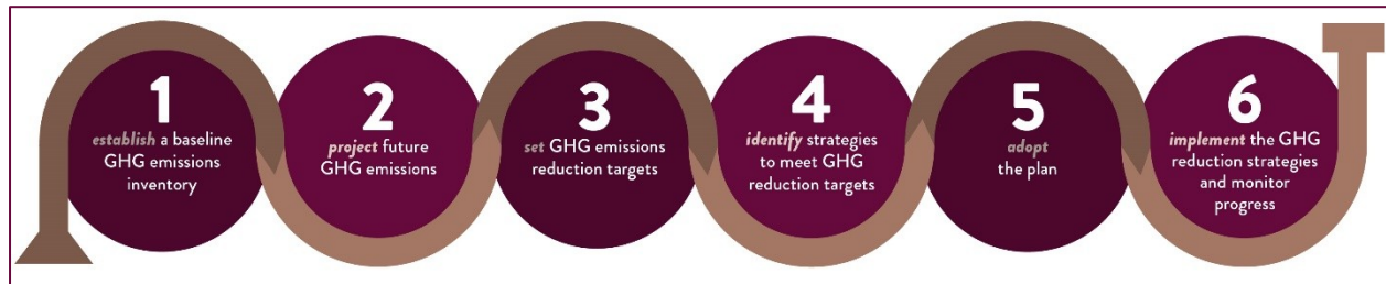
Figure 2.1 Planning Process for Reducing Greenhouse Gas Emissions
